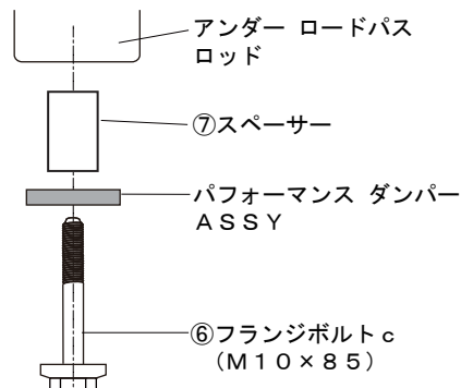
[断面図B]
