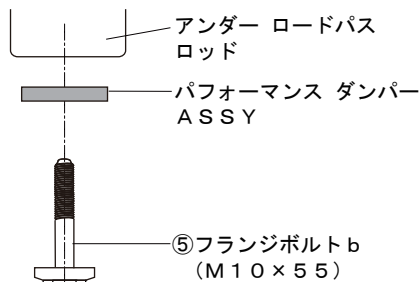
[断面図A]
